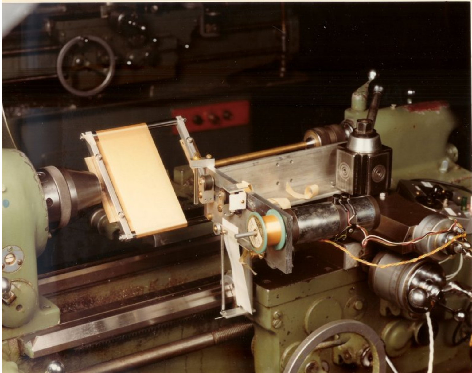
winding polarizers on the lathe
